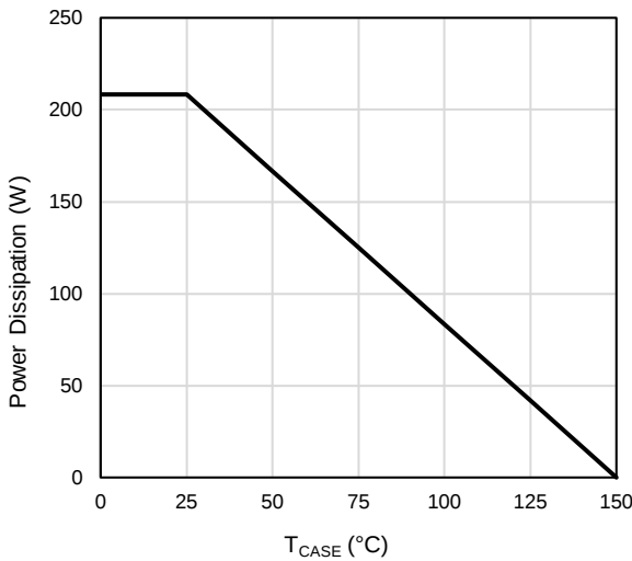
Figure 11: Power De-rating
