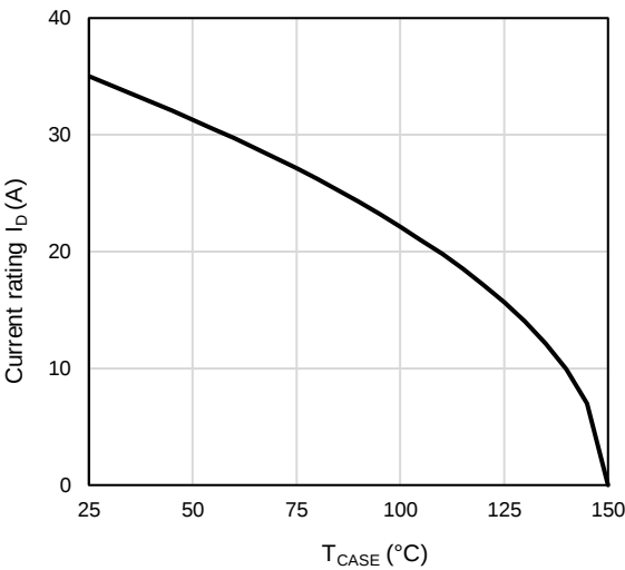
Figure 12: Current De-rating
